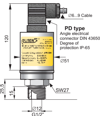
APRE-2000G Economic Version, process connection G1/2" thread (Version with addapter GP. (Designed to measure relative pressure))
