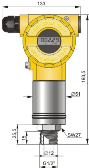
APR-2000GALW, process connection type GP with G1/2" thread. (Designed to measure relative pressure)
