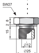
GP type G1/2", Ø12 hole P type M20×1.5, Ø12 hole
