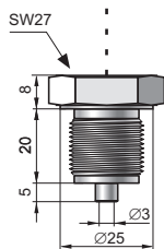
G1/2 type G1/2", Ø3 hole M type M20×1.5, Ø3 hole
