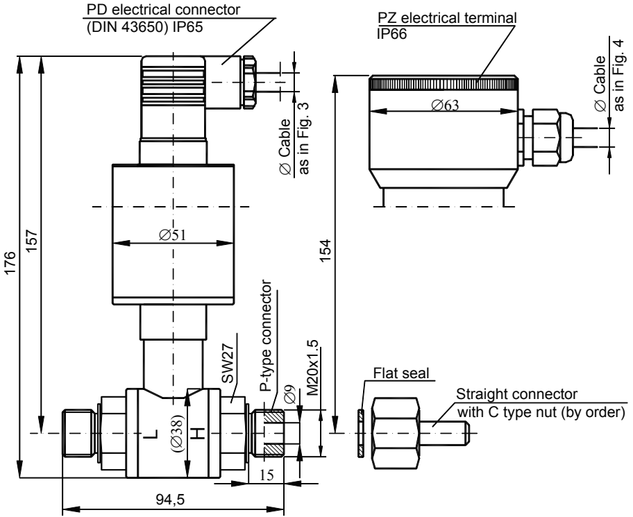
Figure 9. APRE-2000 differential pressure transmitter with P-type connector.
