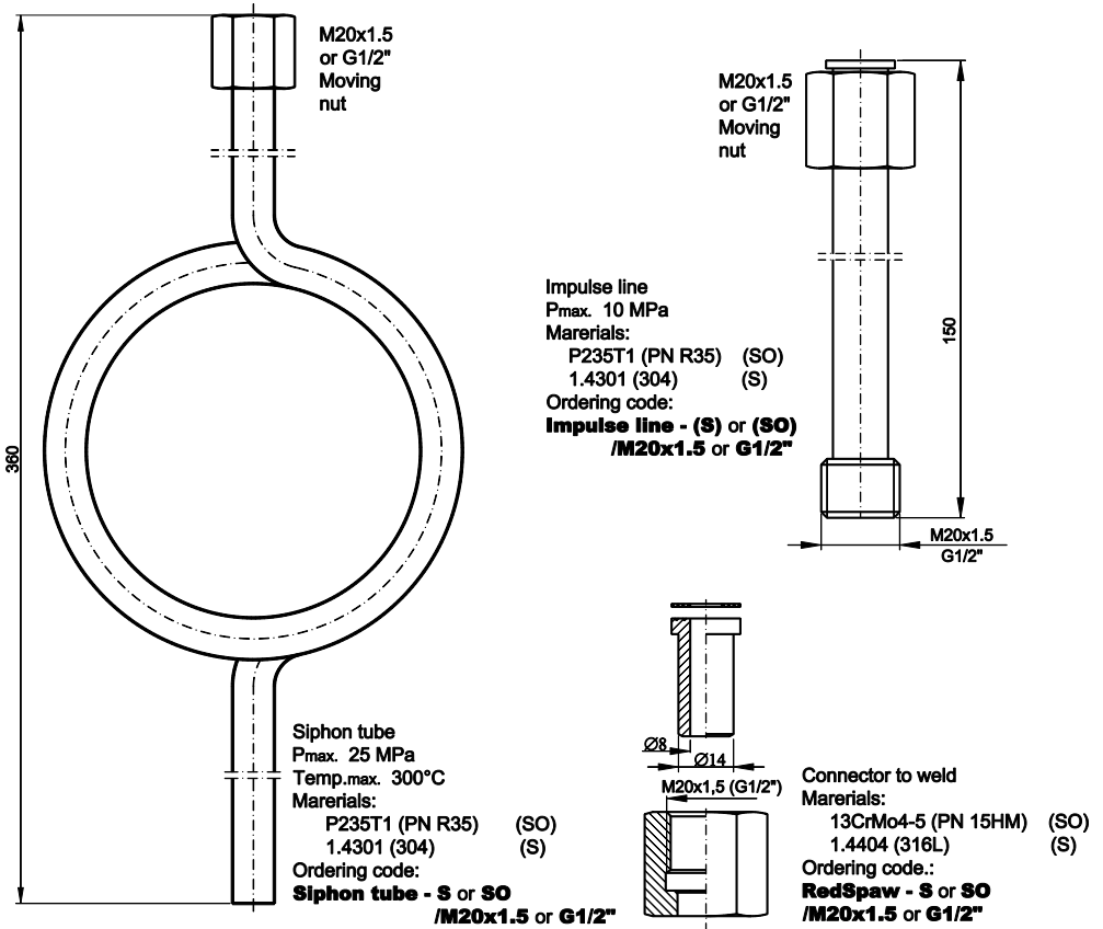
Figure 16. Additional equipment for fitting of pressure transmitters.
