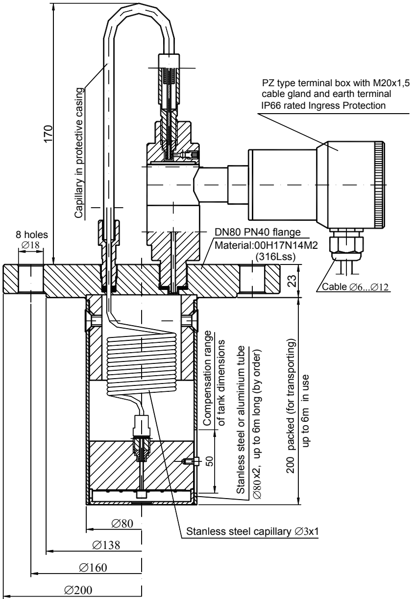
Figure 15. APR-2000Y Smart level probe for pressure tanks.
