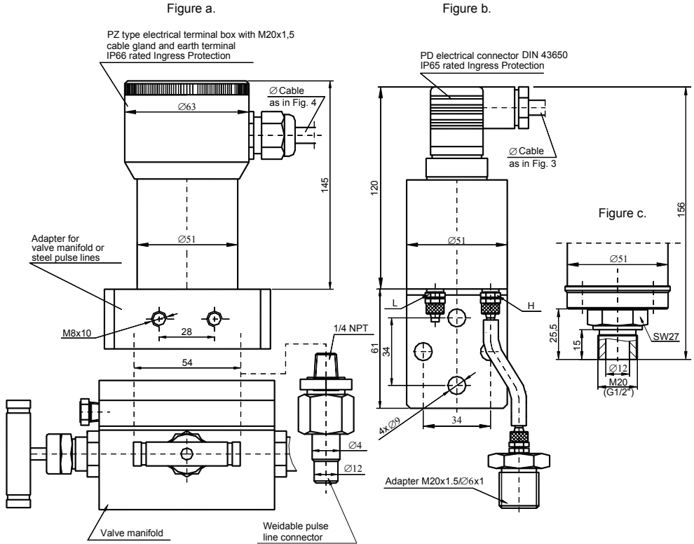
Figure 14. APCE-2000G Smart pressure transmitter and APRE-2000G Smart differential pressure transmitter for low ranges.
