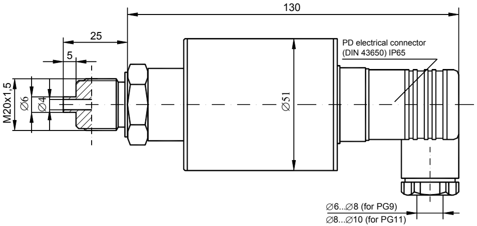
Figure 3. APCE-2000 transmitter with PD connector.
