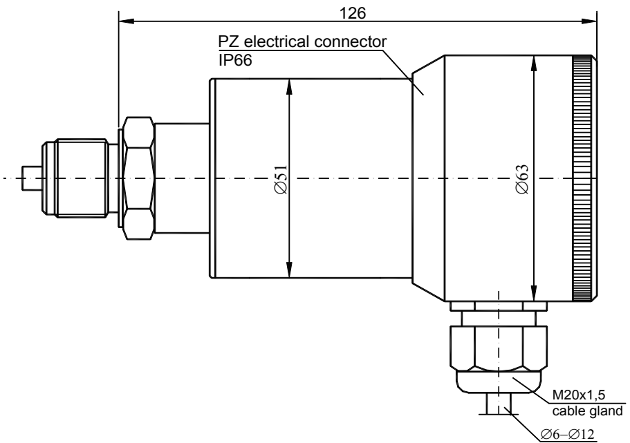
Figure 4. APCE-2000 transmitter with PZ connector.
