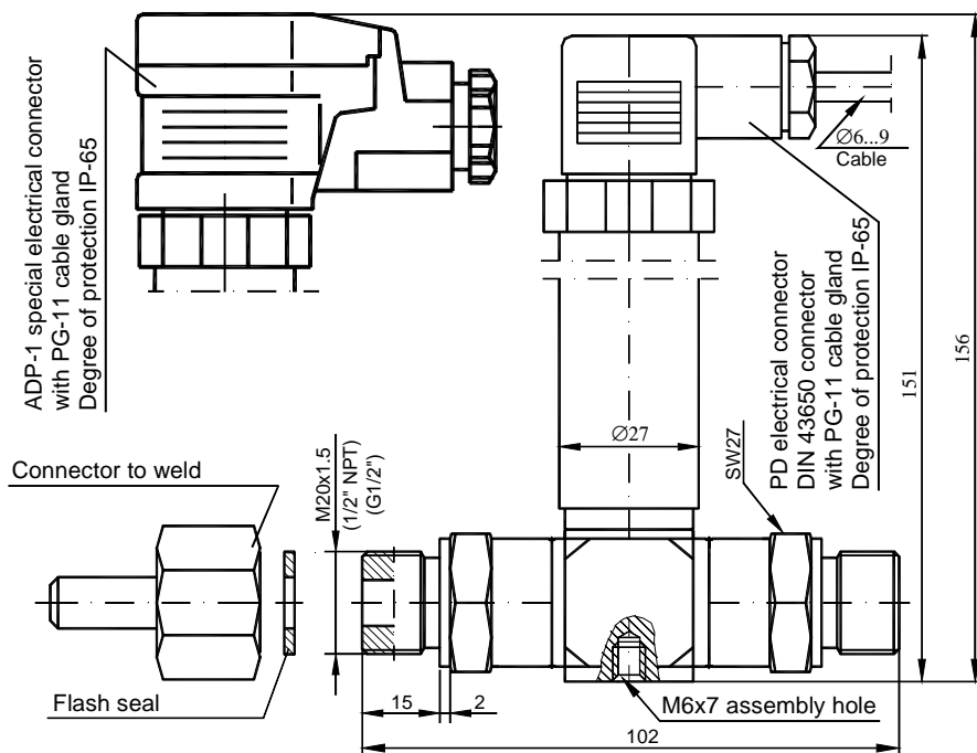
Fig.1. AS-dP series differential pressure transmitter
