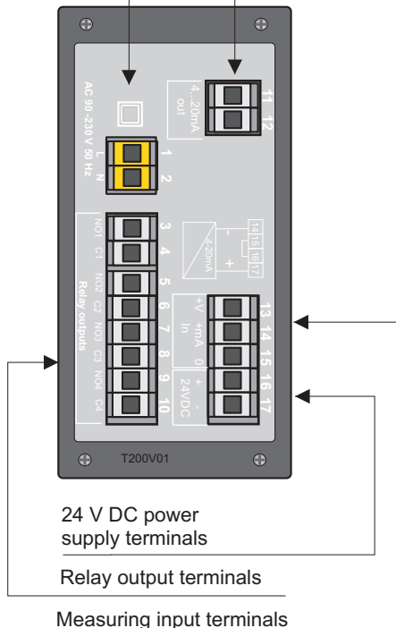
Back side of meter
